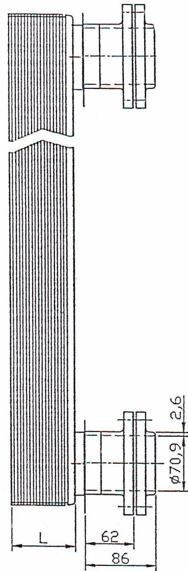
Compac-Flansch DN 65 / PN 40
